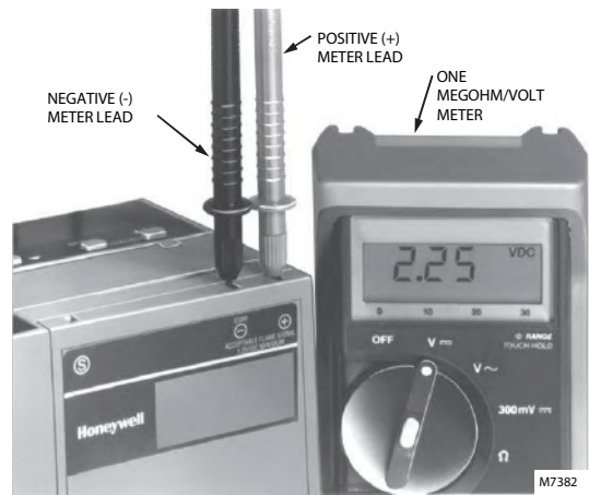
Fig. 11. Measuring voltage flame signal with 7800 Series controls.
